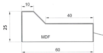
Recessed Rail 'L' Shape
