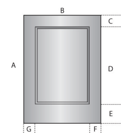
Routed Short Panel
