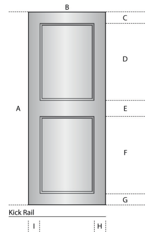
Routed Tall Panel
